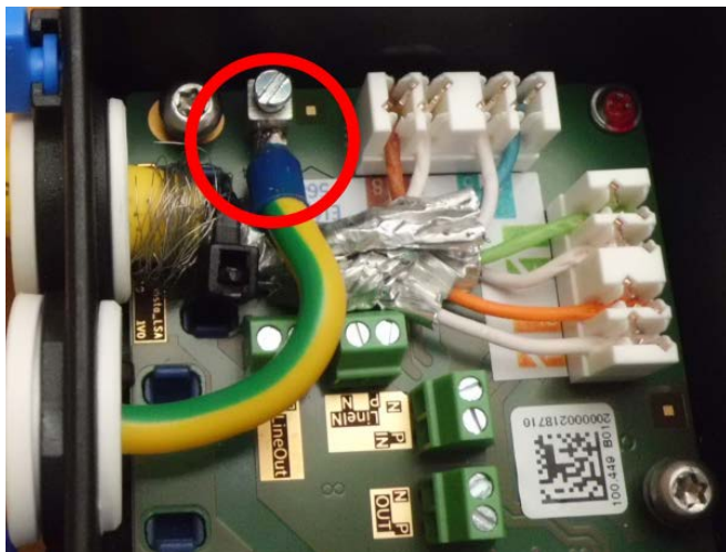
Fig. 30: Ground wire connected to terminal
