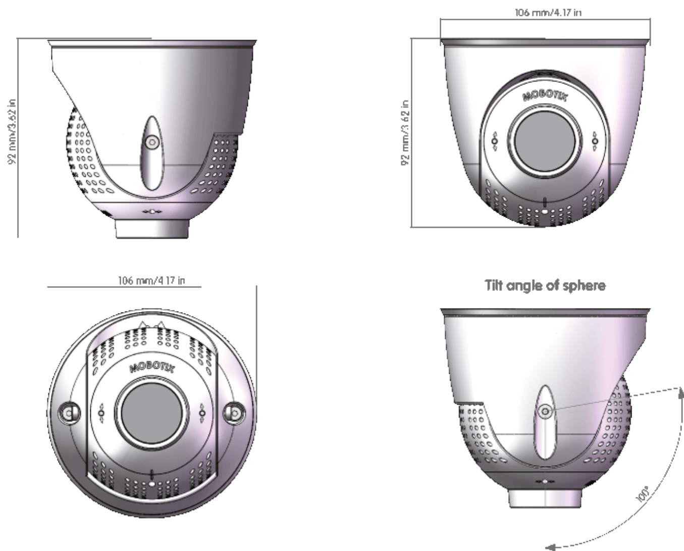
Fig. 3: PTMount-Thermal
