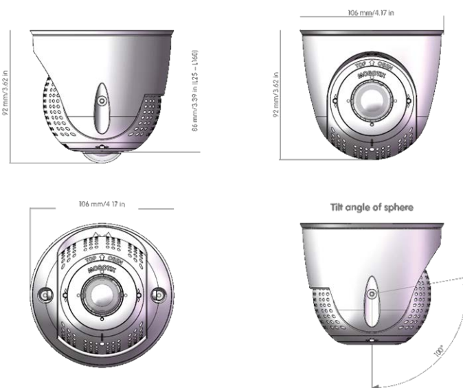
Fig. 2: PTMount
