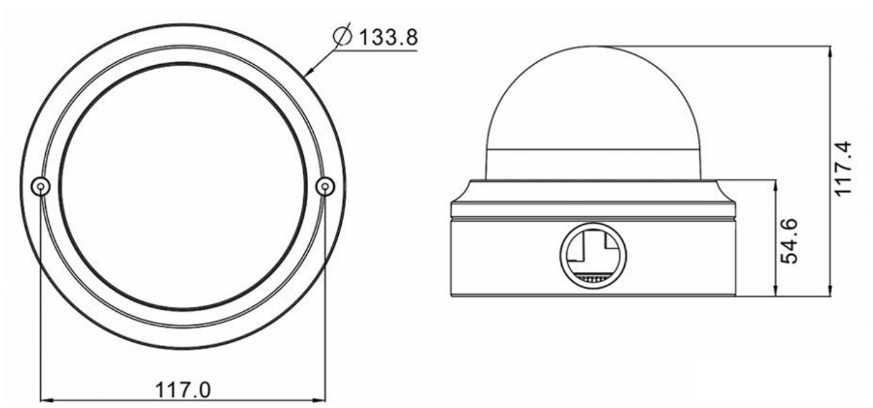
Fig. 1: Mx-VD3A-2-IR-VA: All measurements in mm
